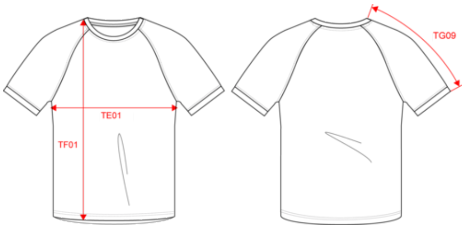
Dimensions (cm)
