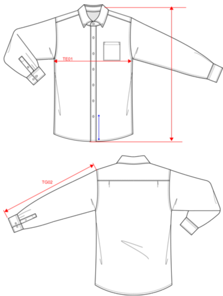
Dimensions (cm)
