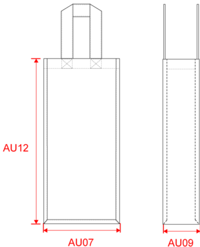
Dimensions (cm)
