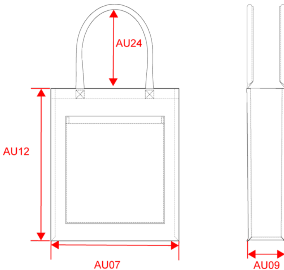
Dimensions (cm)
