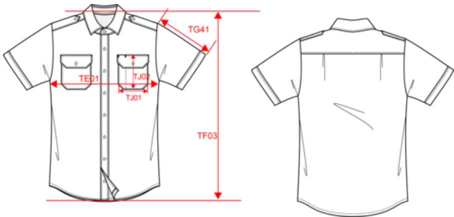
Dimensions (cm)
