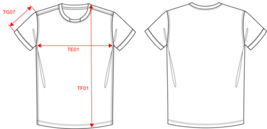
Dimensions (cm)
